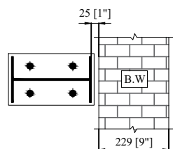
DETAILS = A-A
